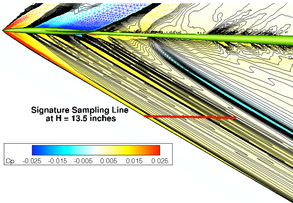
Figure 10: Symmetry plane grid colored by pressure coefficient and overlaid constant pressure lines for USM3D inviscid solution of the SLSLE configuration, M_\infty=2.0 , \alpha=2.3^\circ , H/L=1.5 , Re_L=1.5 million.
