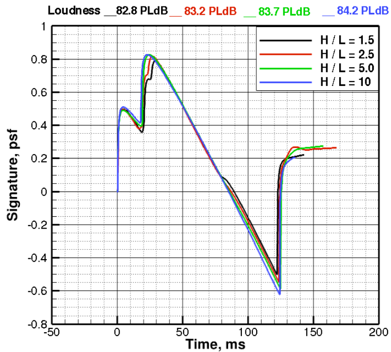
Figure 19: Ground signature sensitivity to separation distance, H/L .
